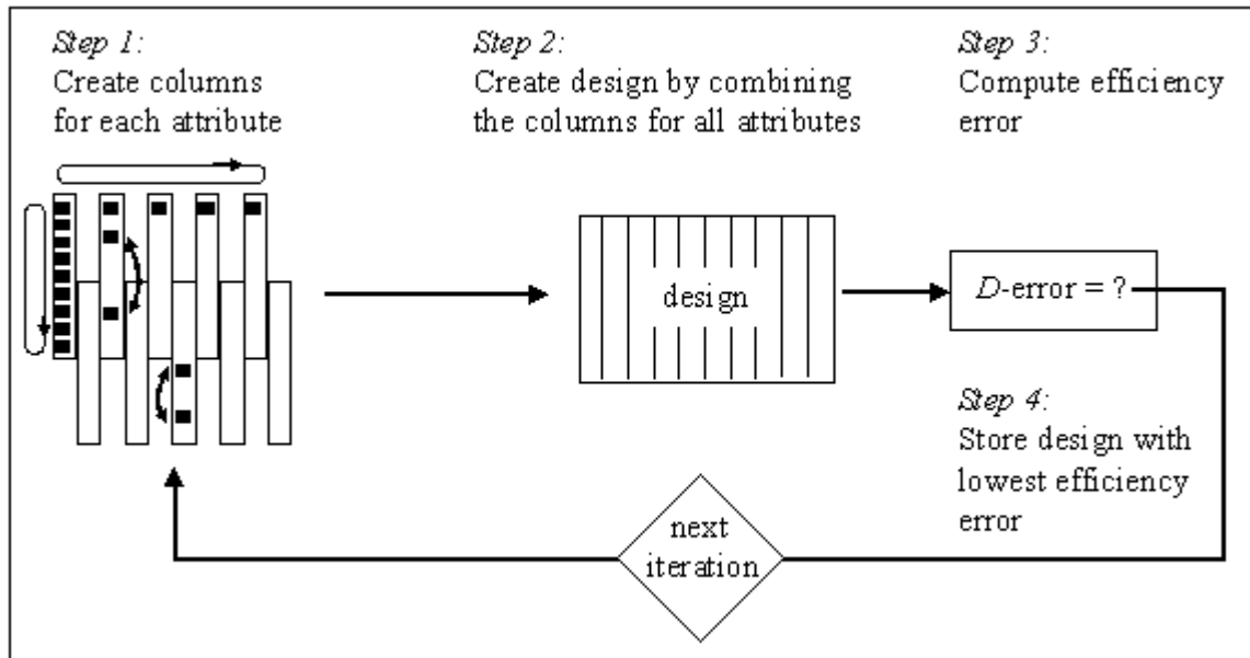
Figure 7.4: RSC algorithm
