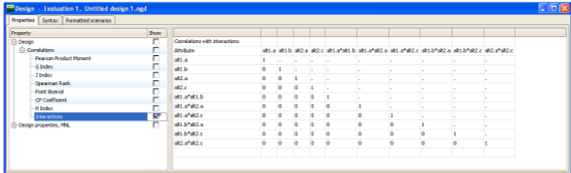
Figure 6.2: Interaction and main effect correlations for a full factorial design output
