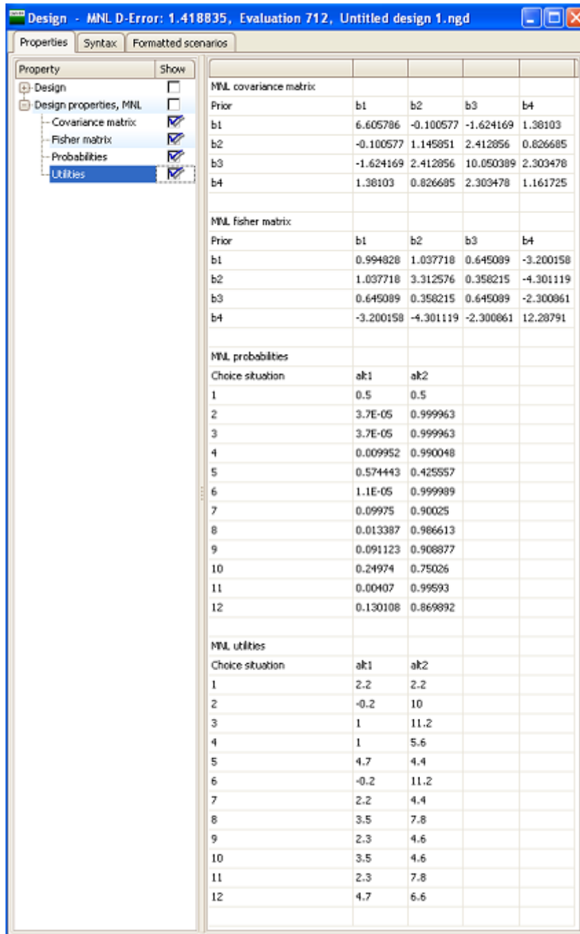
Figure 7.6: Additional MNL design output
