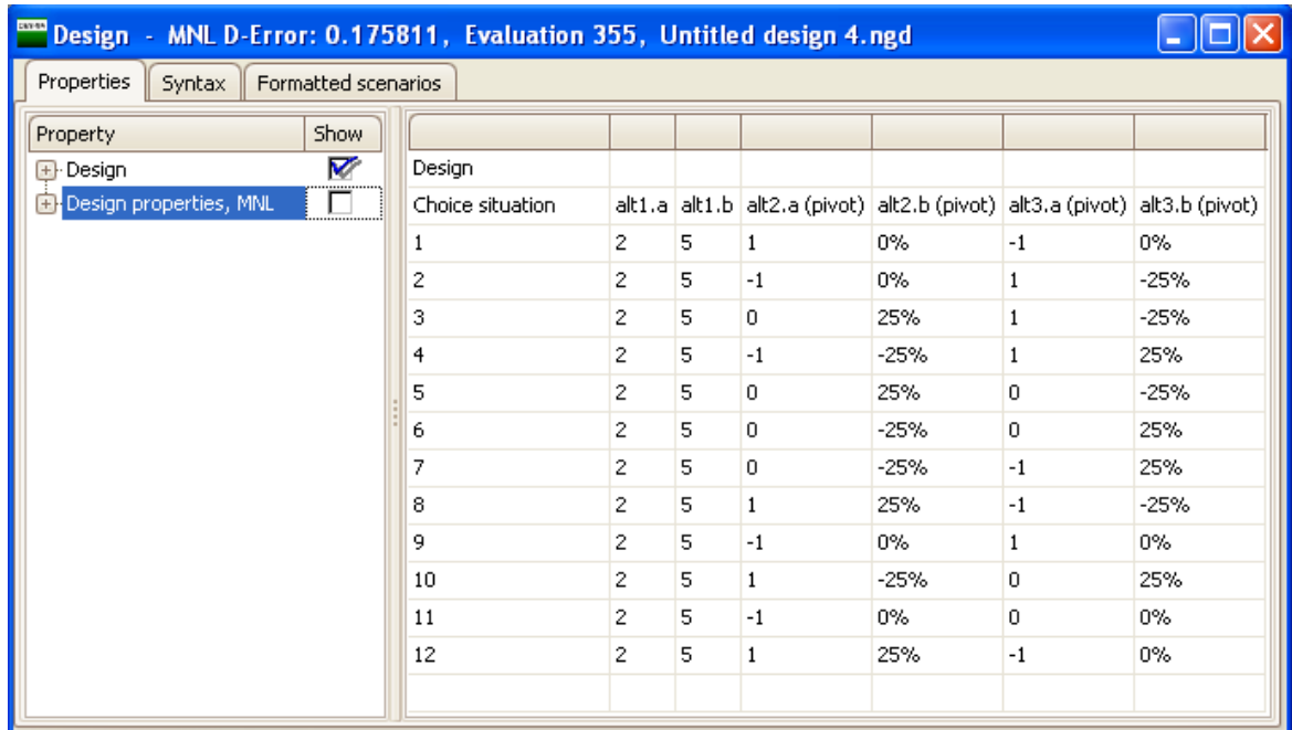
Figure 8.9: Example pivot design assuming everyone observes the same reference alternative (method 2)
