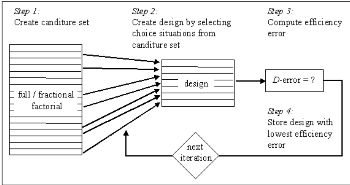
Figure 7.3: Modified Fedorov algorithm
