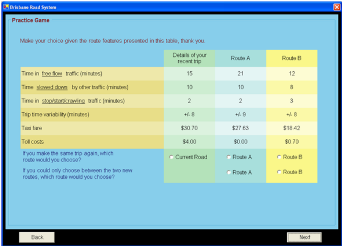
Figure 5.2: Example of a screen in a stated choice experiment
