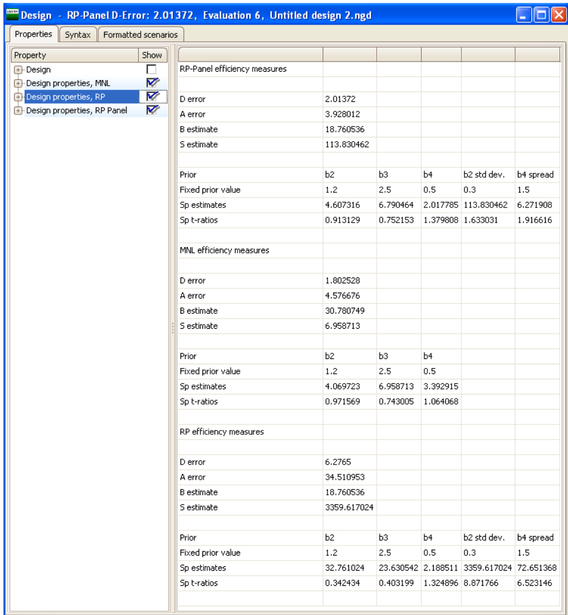
Figure 7.8: MMNL design output by model type
