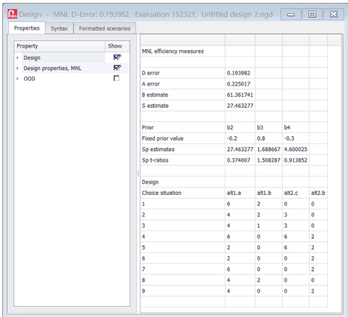
Figure 8.3: A non attribute level balanced design generated with the Modified Fedorov algorithm using Method 2
