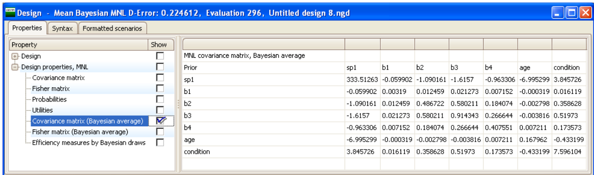
Figure 8.18: Example design output with constrained attribute levels
