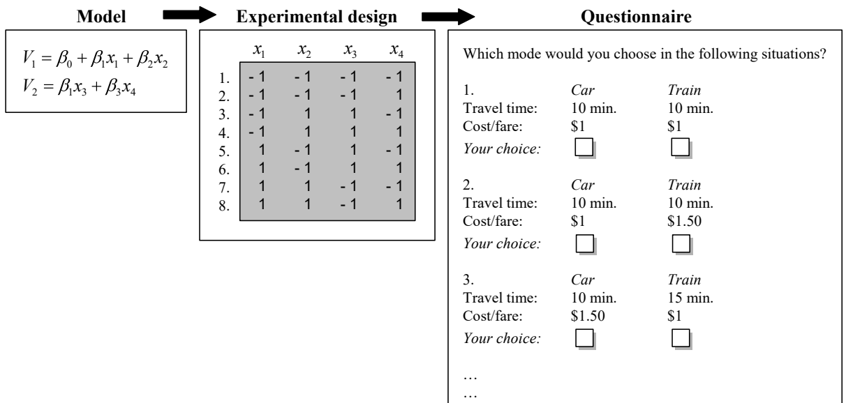
Figure 5.3: Steps in designing a stated choice experiment
