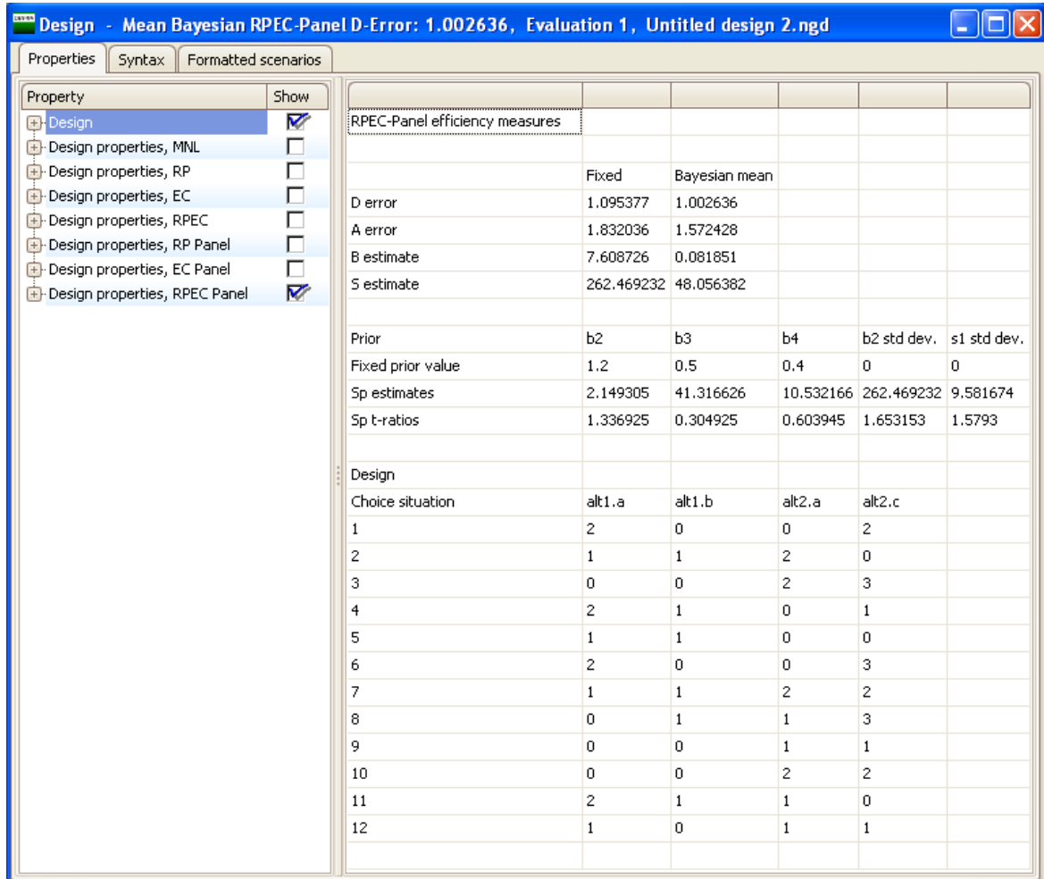
Figure 7.14: Bayesian efficient design output screen
